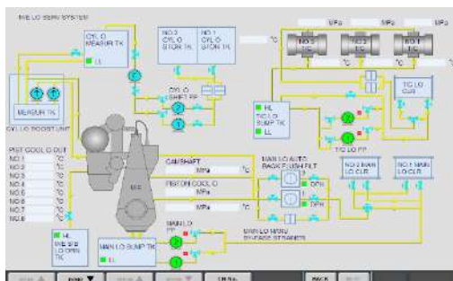
MIMIC screen
